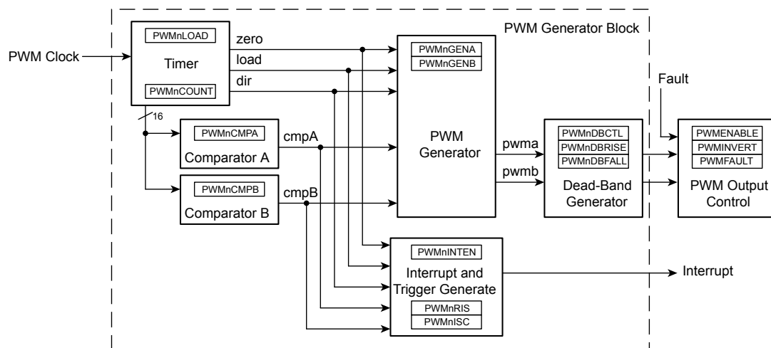
Figure 19-1. PWM Module Block Diagram
