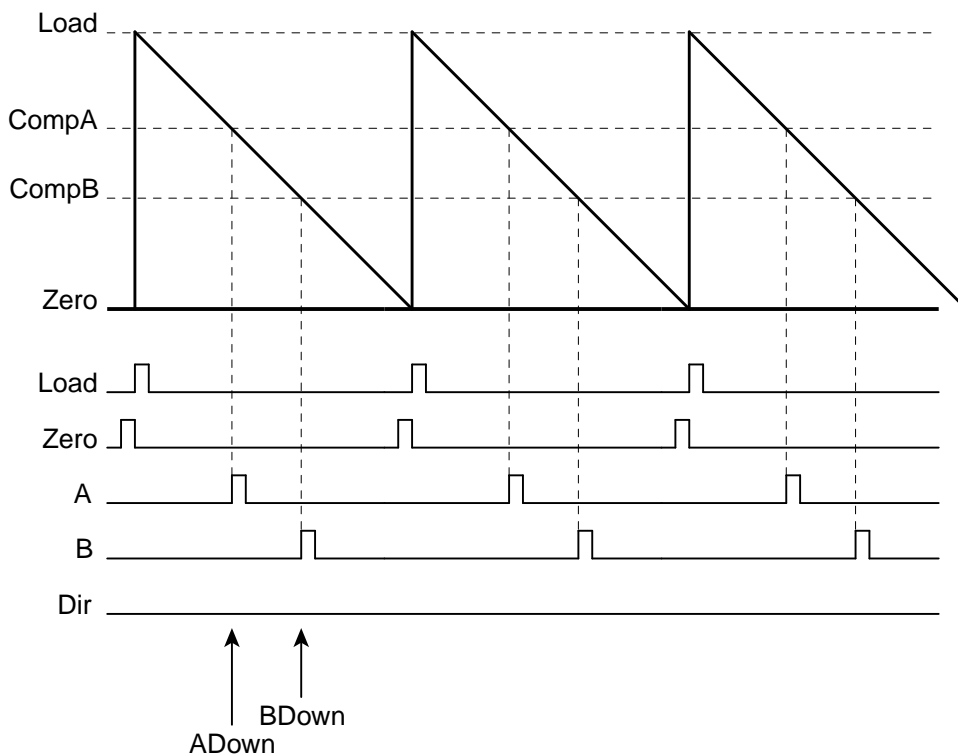
Figure 19-2. PWM Count-Down Mode
