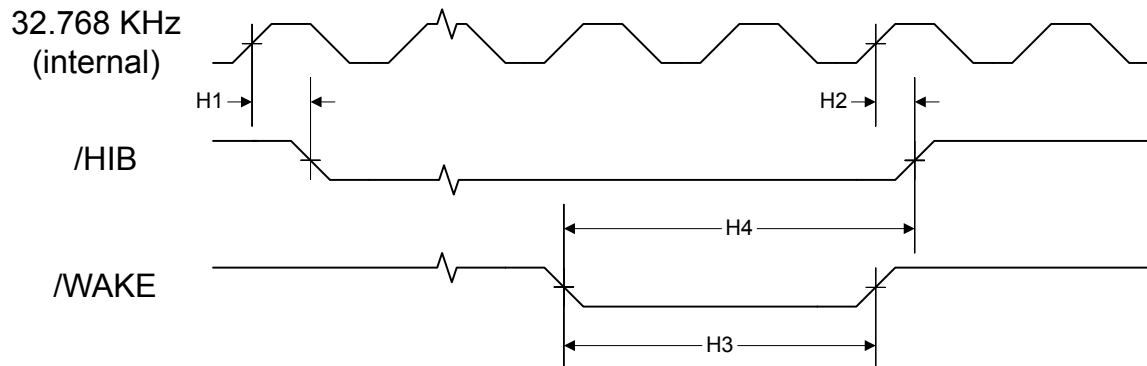
Figure 24-4. Hibernation Module Timing
