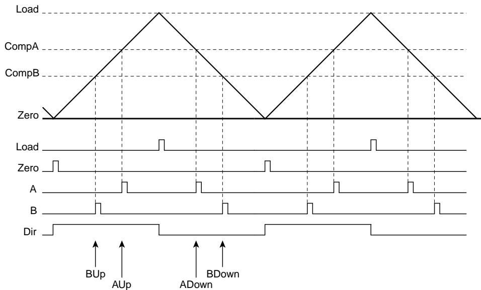
Figure 19-3. PWM Count-Up/Down Mode
