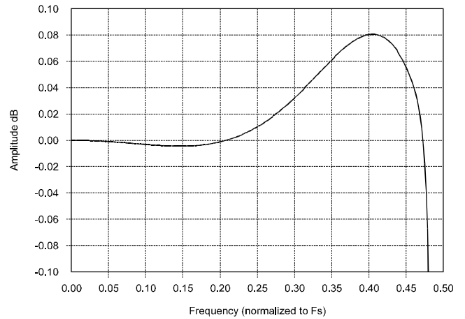
Figure 18. Passband Ripple
