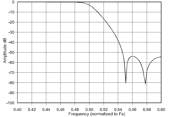
Figure 16. Transition Band
