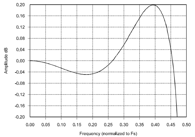
Figure 22. Passband Ripple
