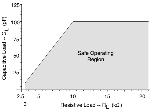
Figure 2. Maximum Loading
