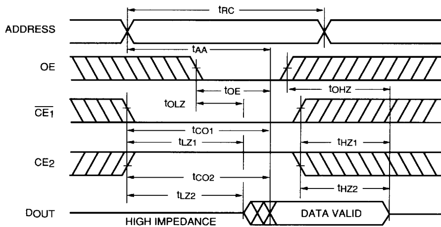
FIGURE 4. READ CYCLE TIMING NO. 2 ( \overline{WE}=V_{IH} )
