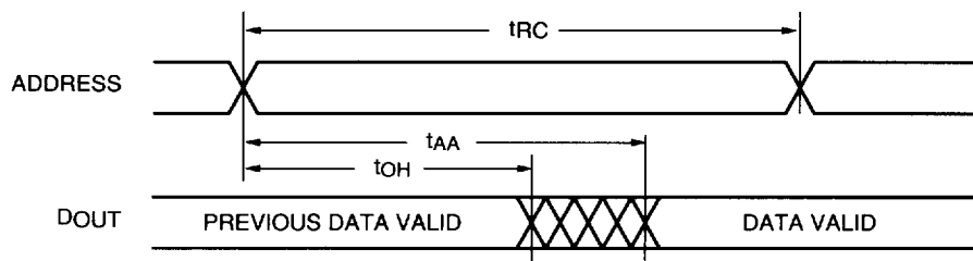
FIGURE 3. READ CYCLE TIMING NO. 1 ( \overline{CS}=\overline{OE}=V_{IL} , \overline{WE}=V_{IH} )
