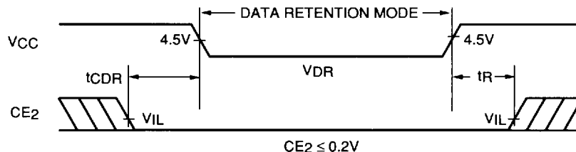
FIGURE 2. LOW V_{CC} DATA RETENTION WAVEFORM ( CE_2 CONTROLLED)
