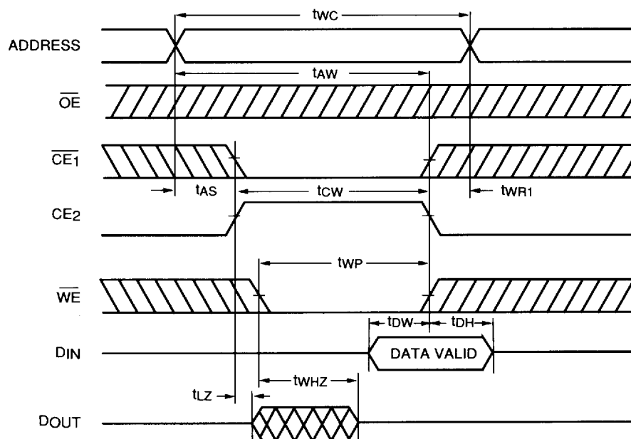
FIGURE 7. WRITE CYCLE TIMING NO. 3 ( CE_2 CONTROL)
