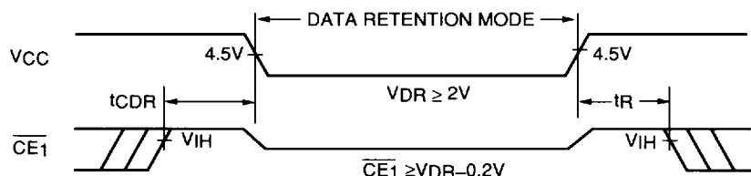
FIGURE 1. LOW V_{CC} DATA RETENTION WAVEFORM ( \overline{CE}_1 CONTROLLED)
