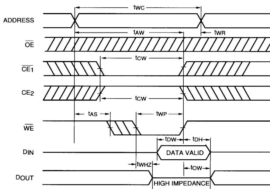
FIGURE 5. WRITE CYCLE TIMING NO. 1 ( \overline{WE} CONTROL)
