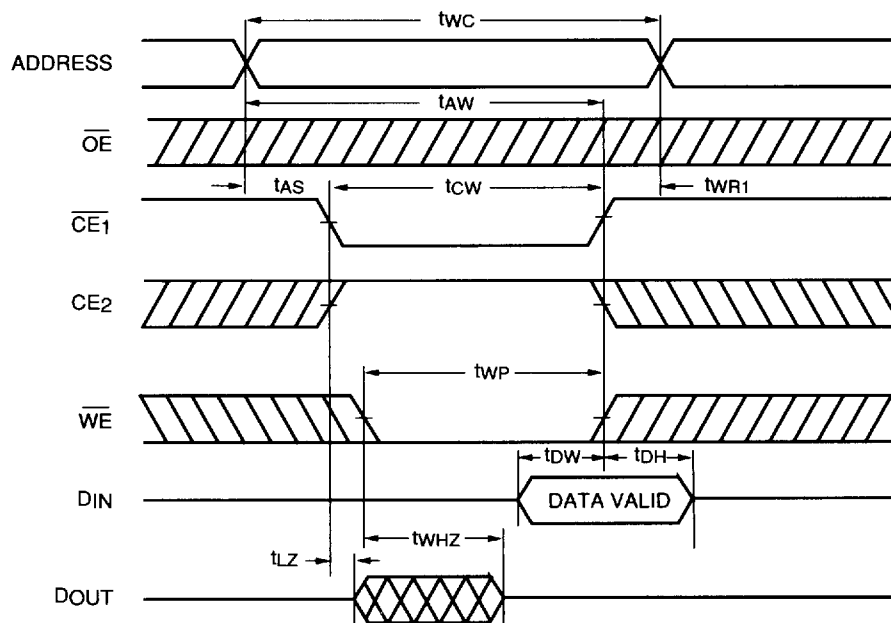
FIGURE 6. WRITE CYCLE TIMING NO. 2 ( \overline{CE}_1 CONTROL)
