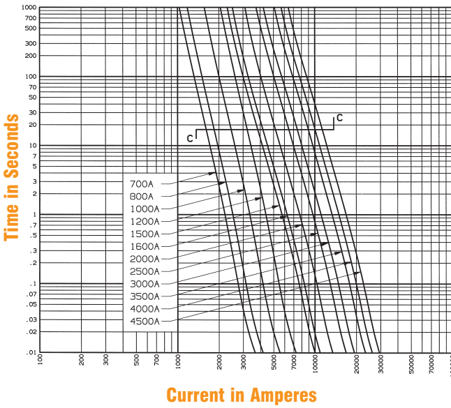
Melting Time - Current Data A30QS 1 to 60
