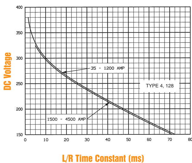
DC Voltage Capability vs. Circuit Time Constant (ms)
