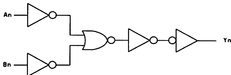
FIGURE 3. Logic diagram.
