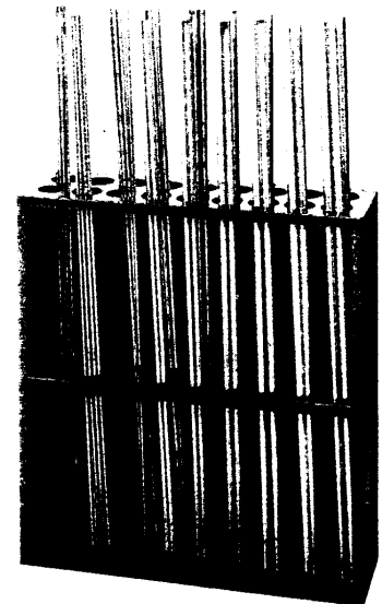
MODEL 367* Threaded Rod Rack. Separates and protects threaded rods. Eighteen 2\frac{1}{8} " diameter openings accommodate different sizes. Shipped fully assembled.
