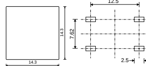
PCB layout
