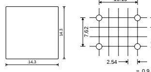
PCB layout
