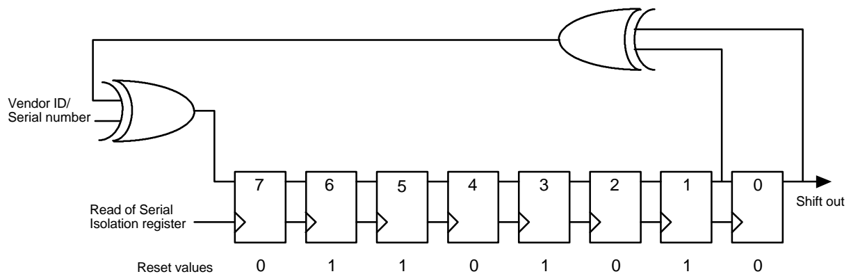
Figure 3. Checksum LFSR
