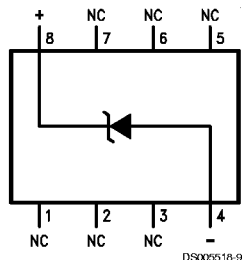
SO Package
