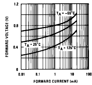
Forward Characteristics
