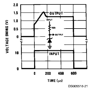
Response Time
