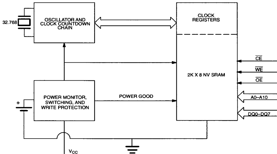
DS1642 BLOCK DIAGRAM Figure 1
