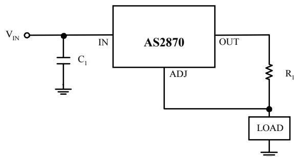
Fig. 4 6.5A Current output Regulator
