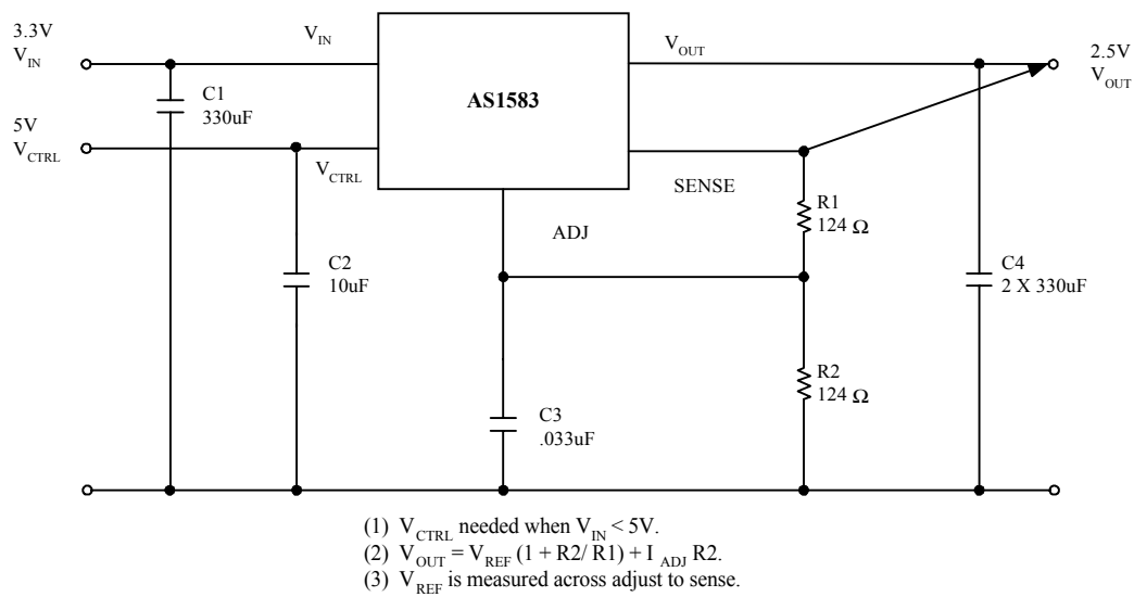
Fig. 1 Adjustable Regulator
