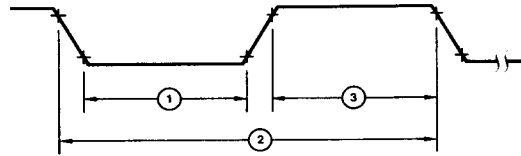
Figure 8. Clock Waveform for All Functions Except Correct Normal or Correct High-Speed
