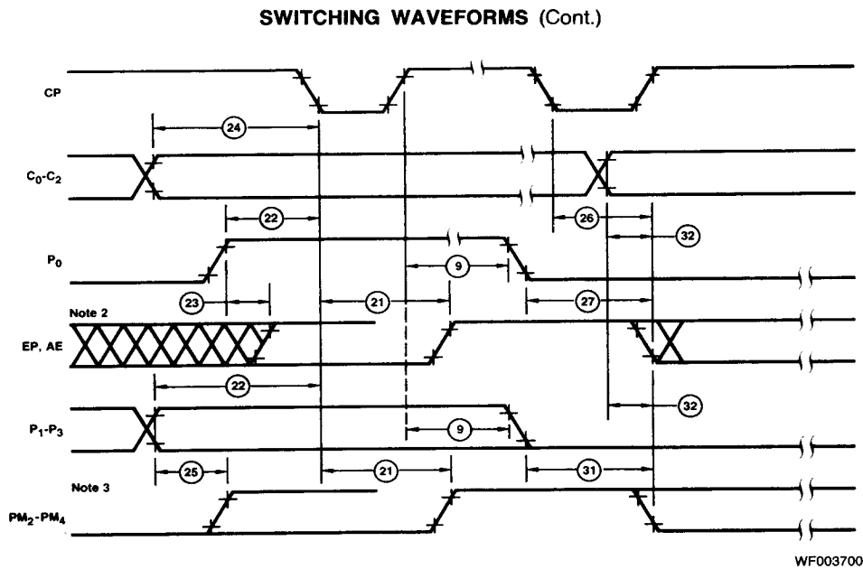
Figure 14. Timing for Correct High-Speed Function
