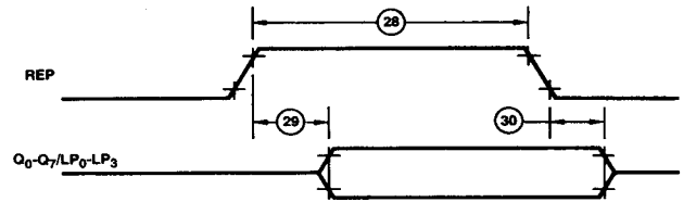
Figure 15. Read Error Pattern Timing
