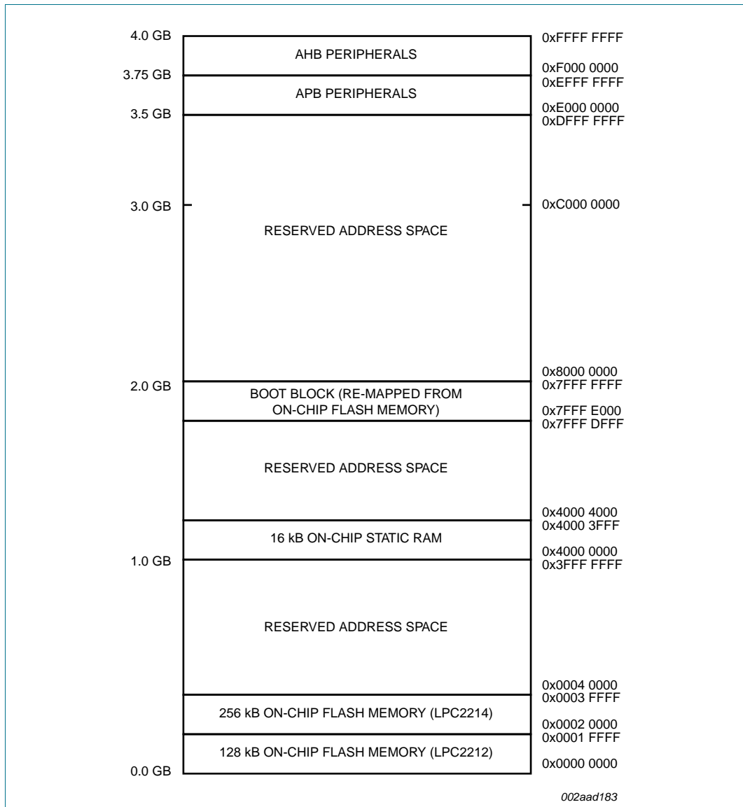
Fig 3. LPC2212/2214 memory map
