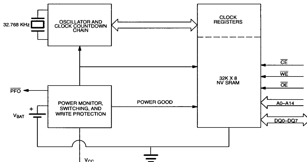
DS1644 BLOCK DIAGRAM Figure 1
