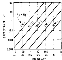
Time Delay vs R_A , R_B and C
