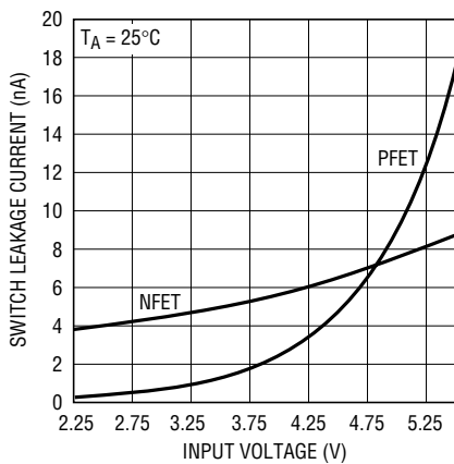
Switch Leakage vs Input Voltage
