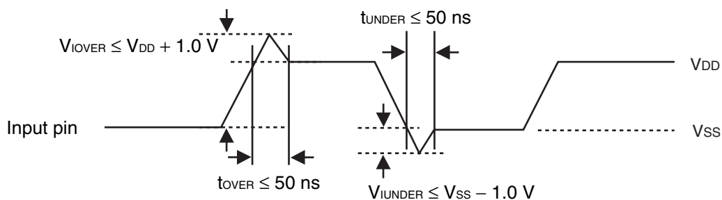
Overshoot/Undershoot
