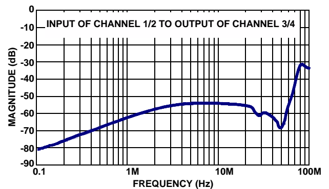
FIGURE 6. INTER-CHANNEL CROSSTALK
