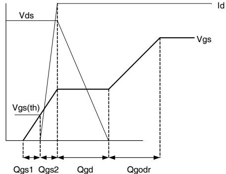
Fig 24b. Gate Charge Waveforms
