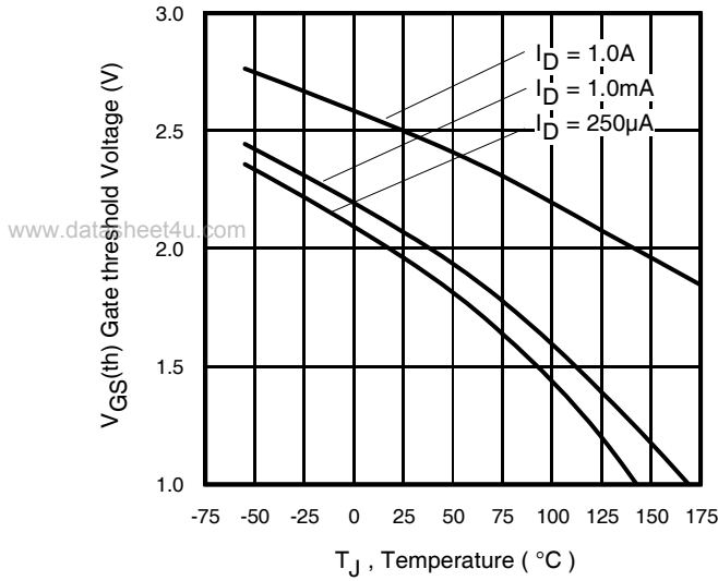
Fig 16. Threshold Voltage Vs. Temperature
