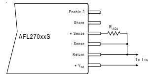
Figure V. Connection for V_{OUT} Adjustment
