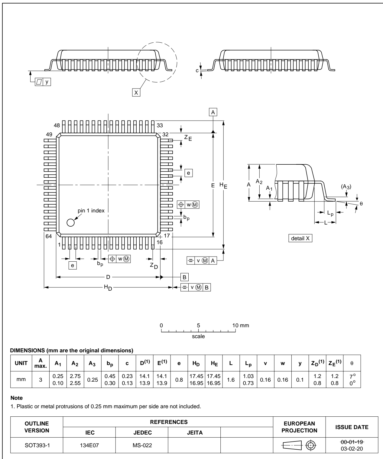
Fig 42. Package outline SOT393-1 (QFP64)
