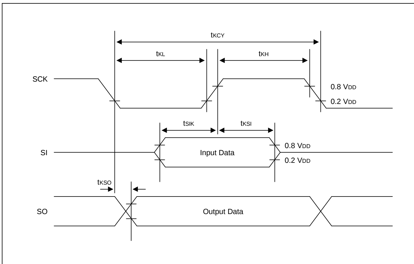
Figure 15-10. Serial Data Transfer Timing
