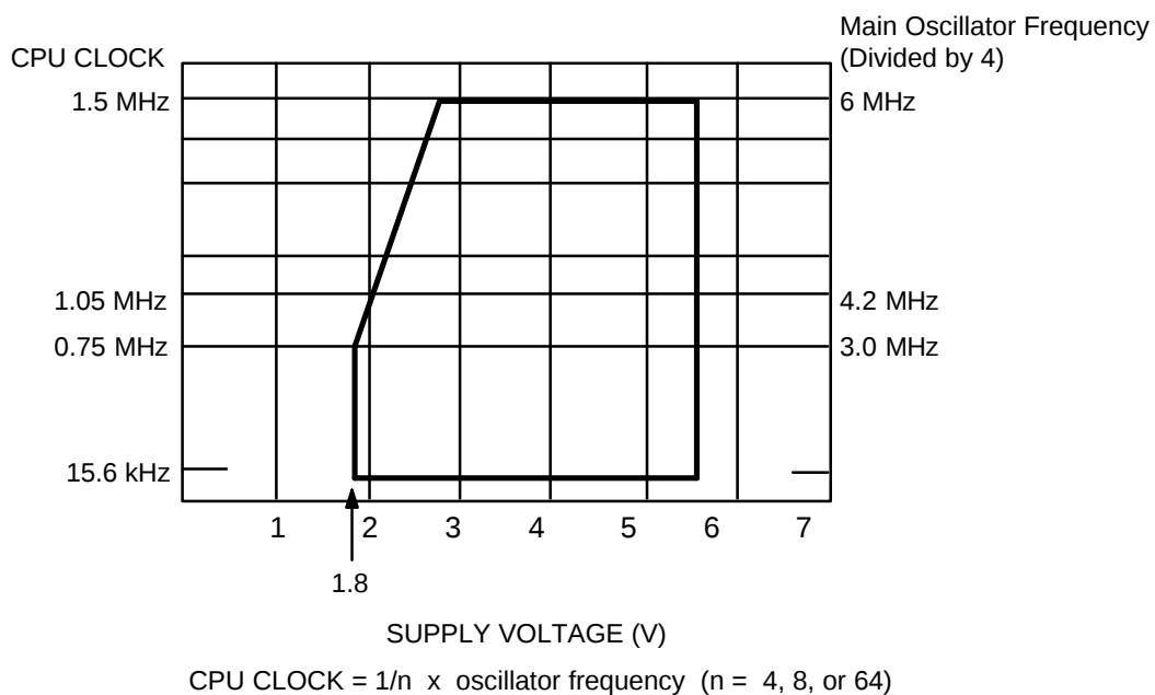
Figure 15-1. Standard Operating Voltage Range
