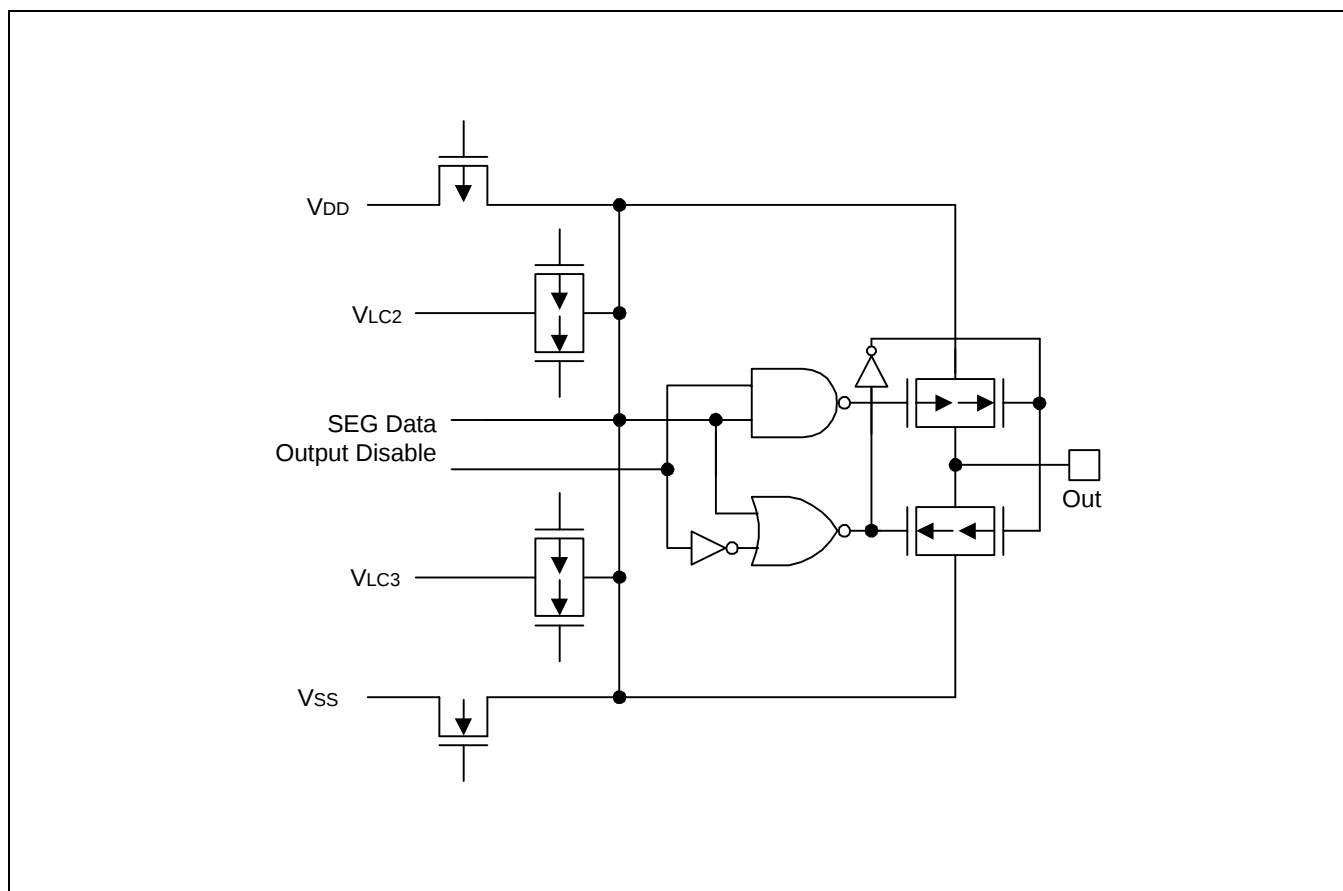
Figure 1-11. Pin Circuit Type H-7
