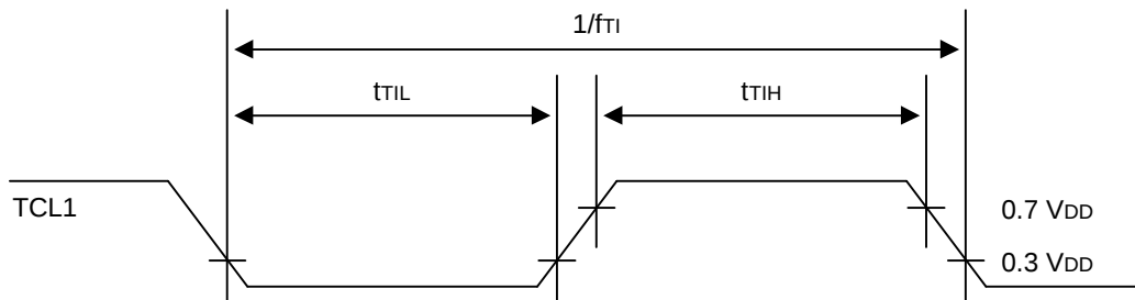
Figure 15-7. TCL1 Timing
