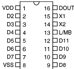
HT12C -16 DIP/SOP
