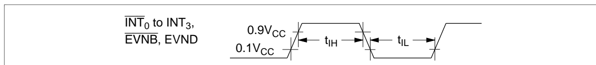
Figure 95 Interrupt Timing
