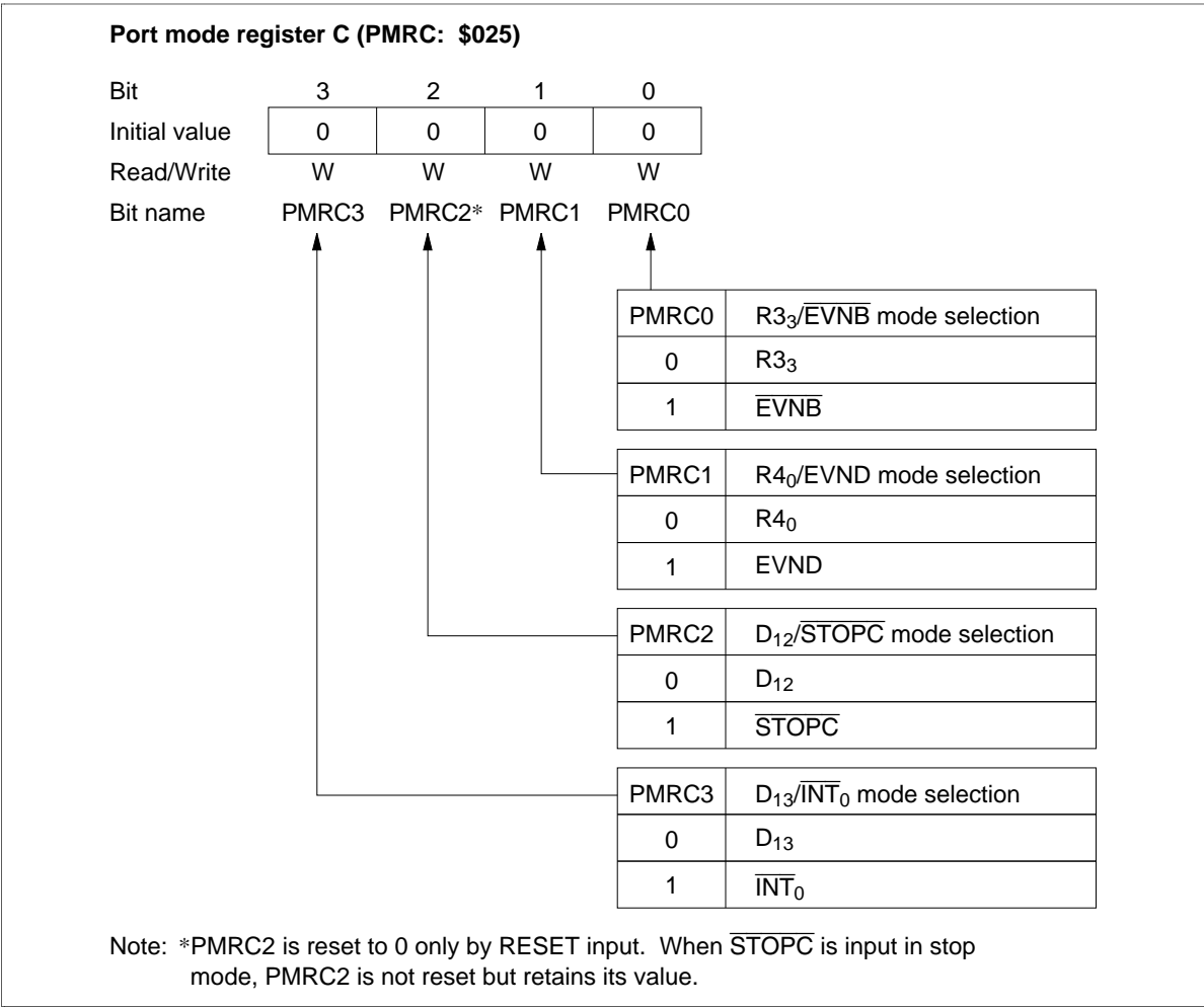
Figure 30 Port Mode Register C (PMRC )
