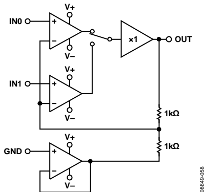
Figure 56. Conceptual Diagram of ADV3220
