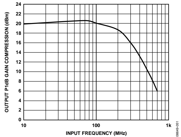
Figure 49. ADV3220 Output P1dB Gain Compression, R_L = 100 \Omega , C_L = 4 \text{ pF}
