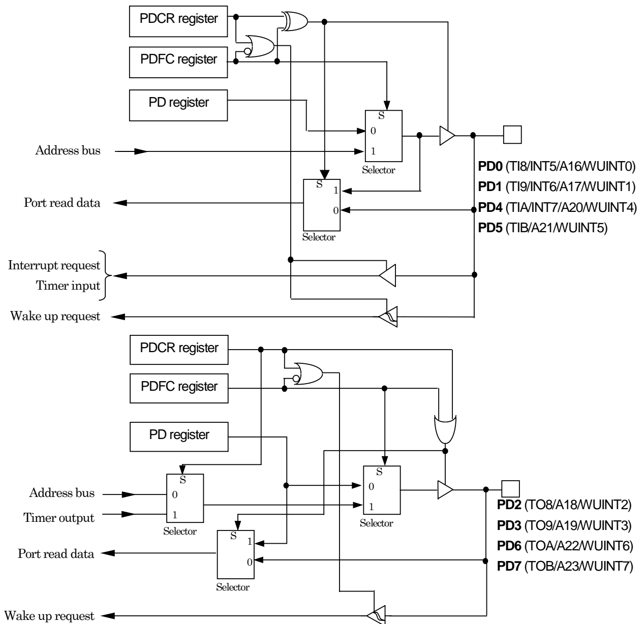
Figure 3.5.6 PortD
