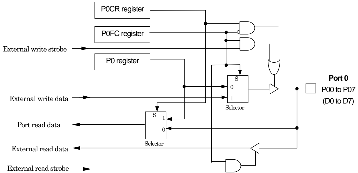
Figure 3.5.1 Port0
