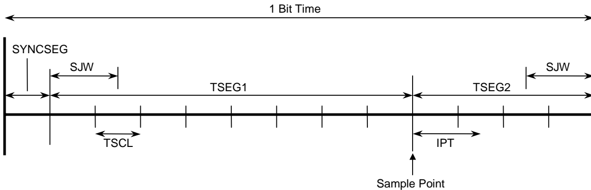
Figure 3.12.3 Bit Timing
