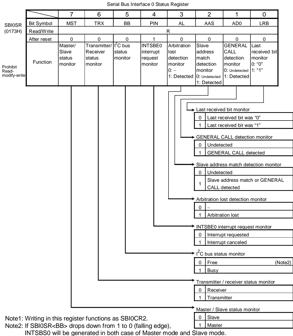
Figure 3.10.5 Registers for the I 2 C Bus Mode
