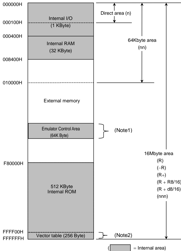
Figure 3.2 Memory Map
