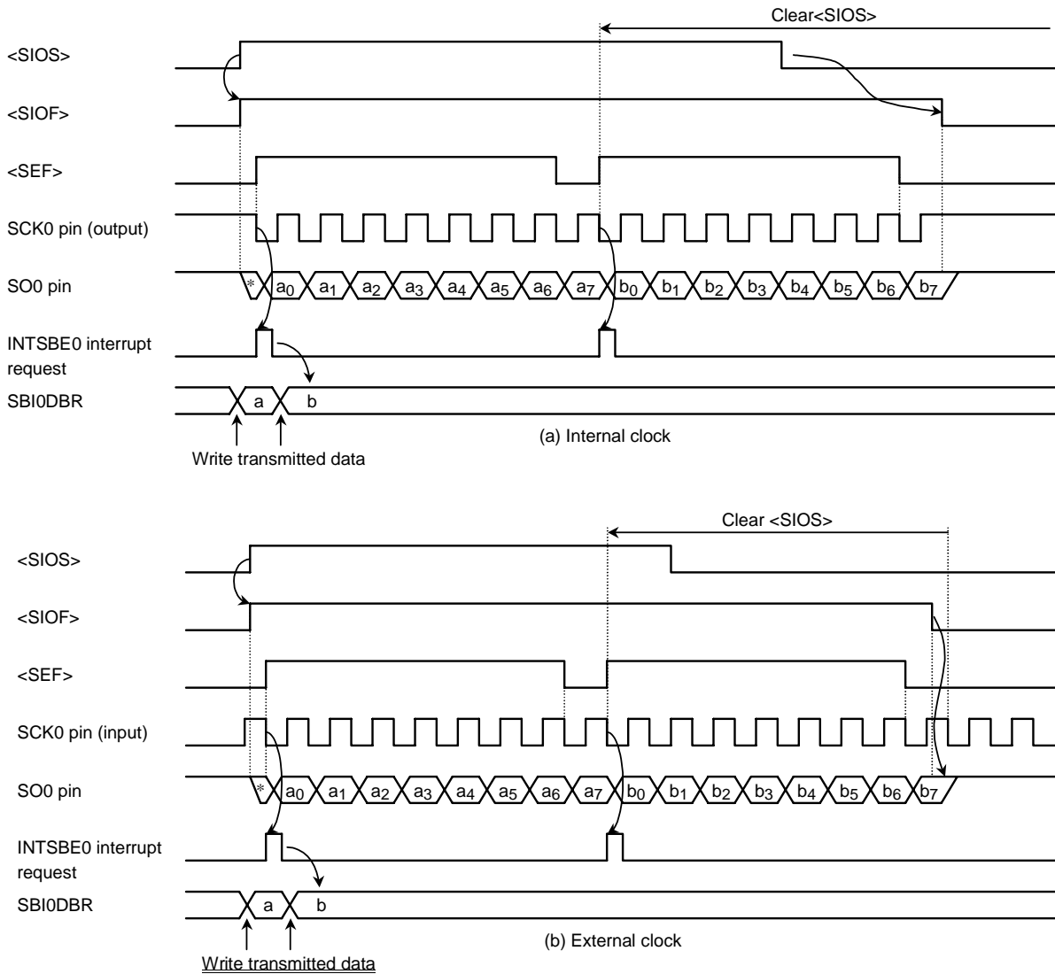
Figure 3.10.39 Transfer Mode
