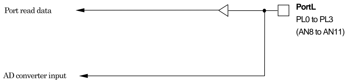
Figure 3.5.10 PortL
