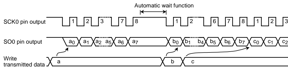
Figure 3.10.36 Automatic-wait Function
