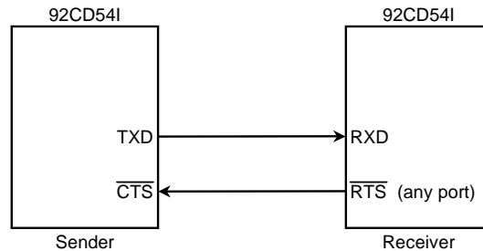
Figure 3.9.6 Handshake function
