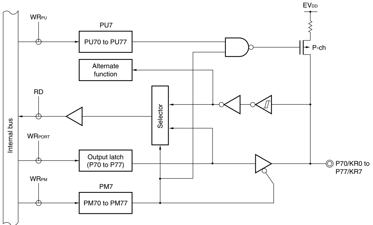
Figure 4-14. Block Diagram of P70 to P77
