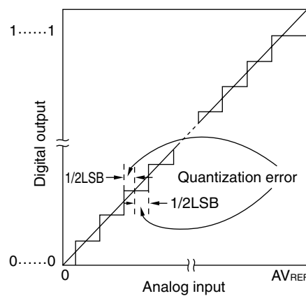
Figure 12-13. Quantization Error
