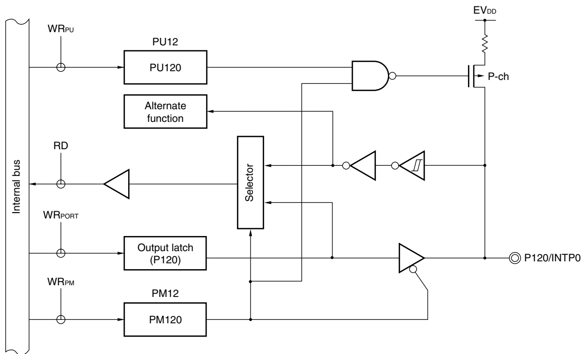
Figure 4-15. Block Diagram of P120
