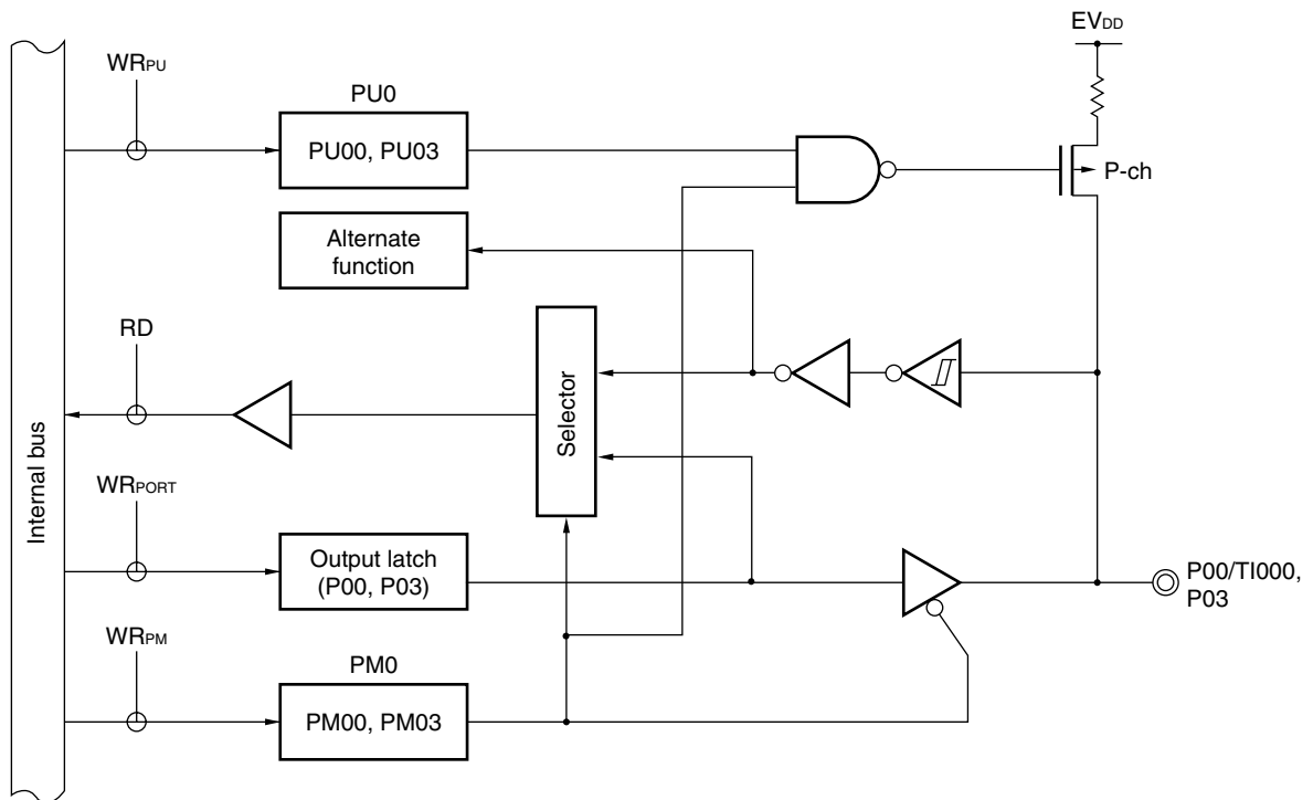
Figure 4-2. Block Diagram of P00 and P03
