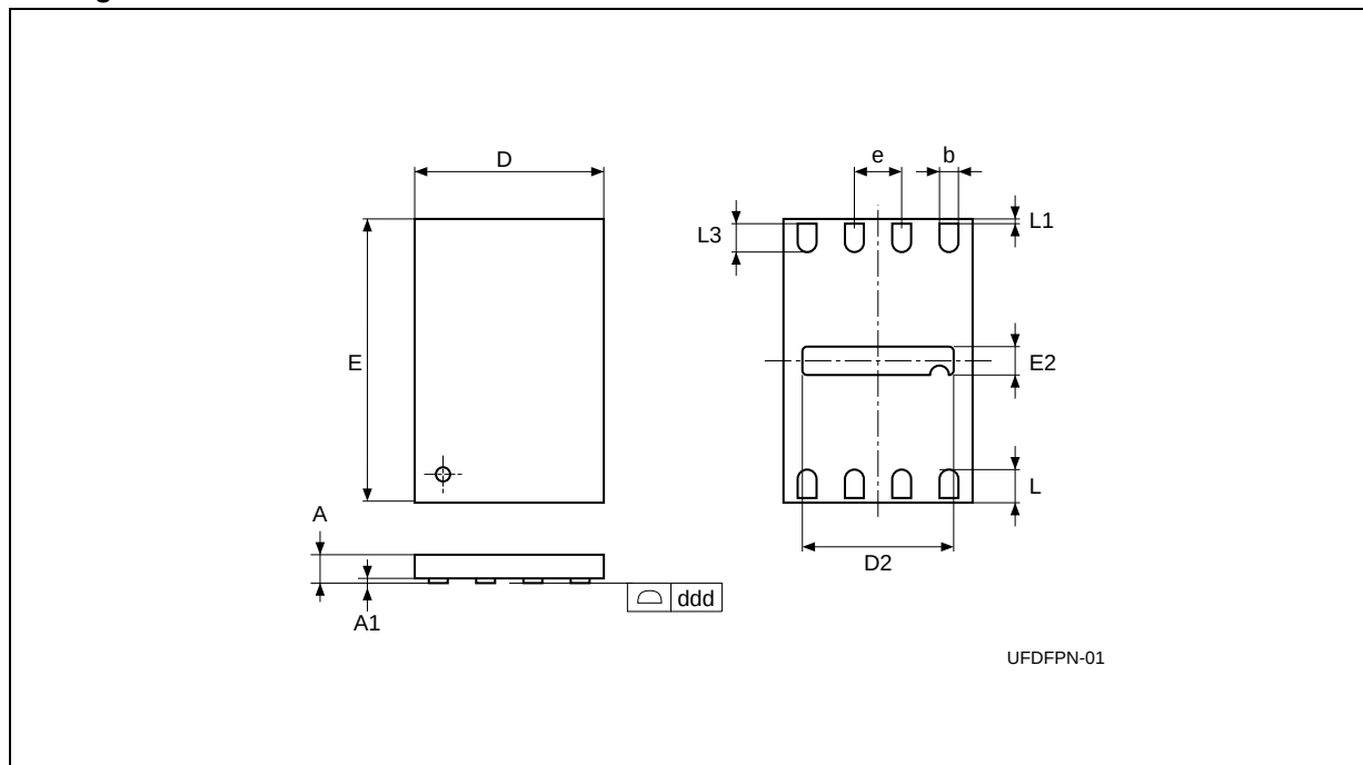
Figure 14. UDFPN8 (MLP8) 8-lead Ultra thin Fine pitch Dual Flat Package No lead 2x3mm 2 , Package Outline
