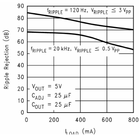
B2117-ADJ Ripple Rejection vs. Current
