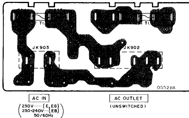
I AC IN/AC OUTLET P.C.B. FOR [E,EB,EG] AREAS.
