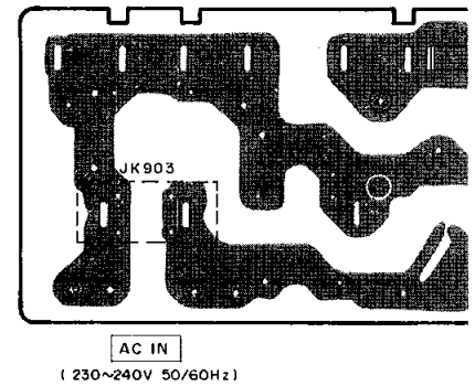
I AC IN/AC OUTLET P.C.B. FOR [G]
