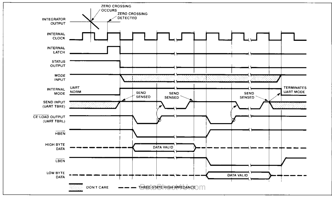
Figure 10. Handshake - Typical UART Interface Timing
