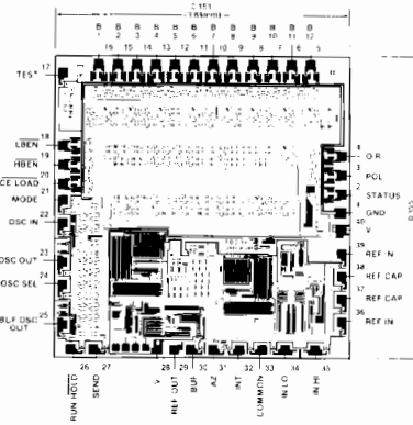
Chip Topography
