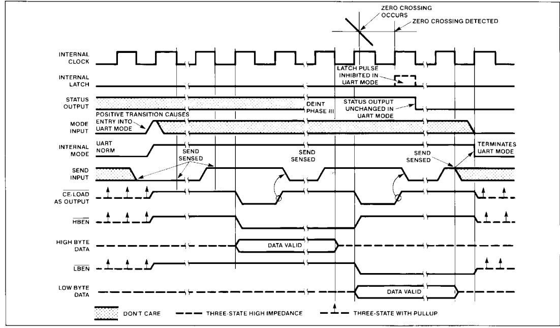
Figure 11. Handshake Triggered By Mode
