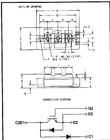
CM200E3Y-12E Outline Drawing
