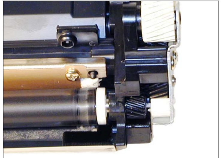
Install the cleaned developer roller in the hopper keyed end first. Spin it until it is fully seated in the drive gear.
