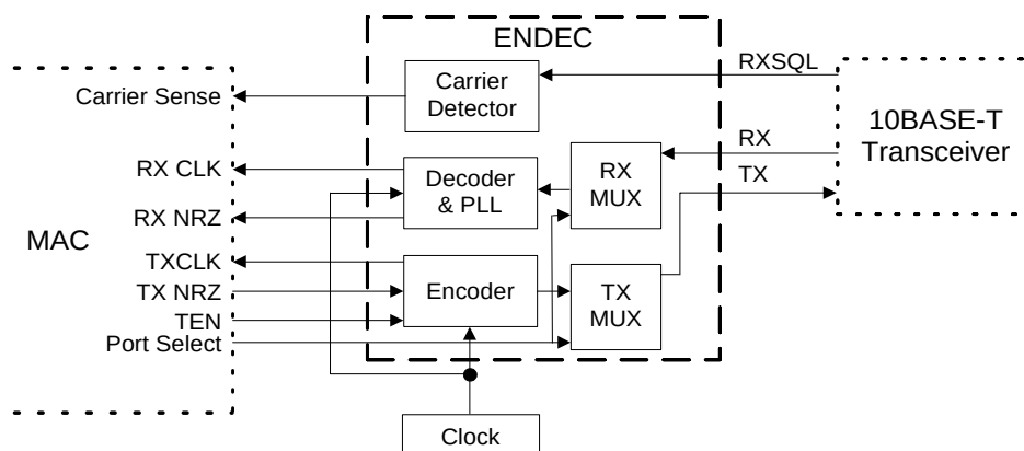
Figure 16. ENDEC
