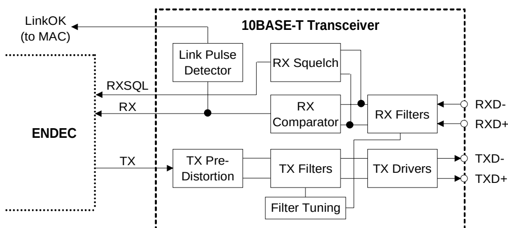
Figure 17. 10BASE-T Transceiver
