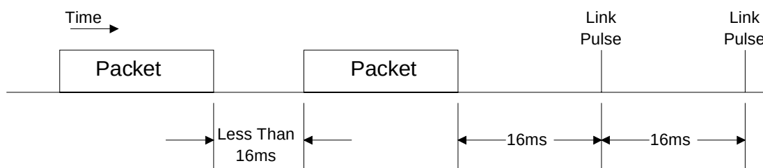
Figure 18. Link Pulse Transmission
