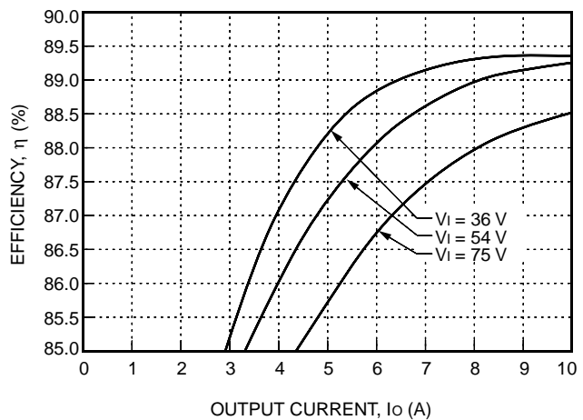
Figure 12. Typical JFW150C Converter Efficiency vs. Output Current at Room Temperature
