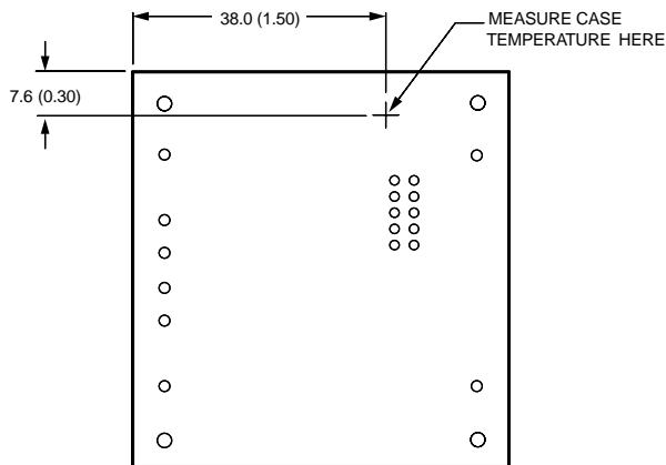
Figure 27. Case Temperature Measurement Location
