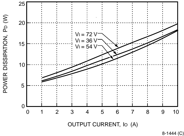
Figure 32. JFW150C Power Dissipation vs. Output Current
