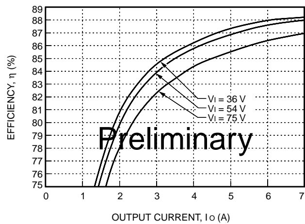
Figure 11. Typical JFW100C Converter Efficiency vs. Output Current at Room Temperature
