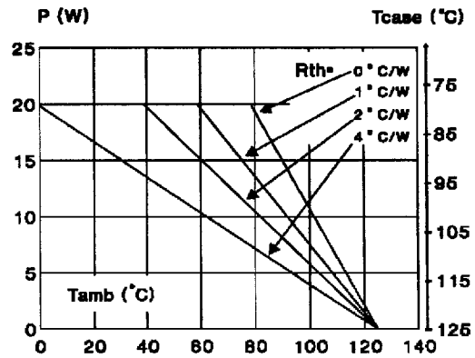
Fig.2 : Correlation between maximum RMS power dissipation and maximum allowable temperatures ( T_{amb} and T_{case} ) for different thermal resistances heatsink + contact (BTA).
