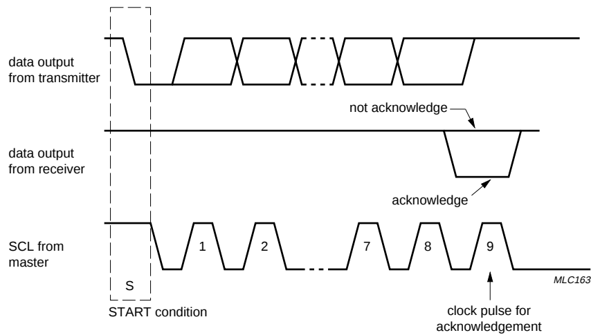
Fig.15 Acknowledge on the I 2 C-bus.
