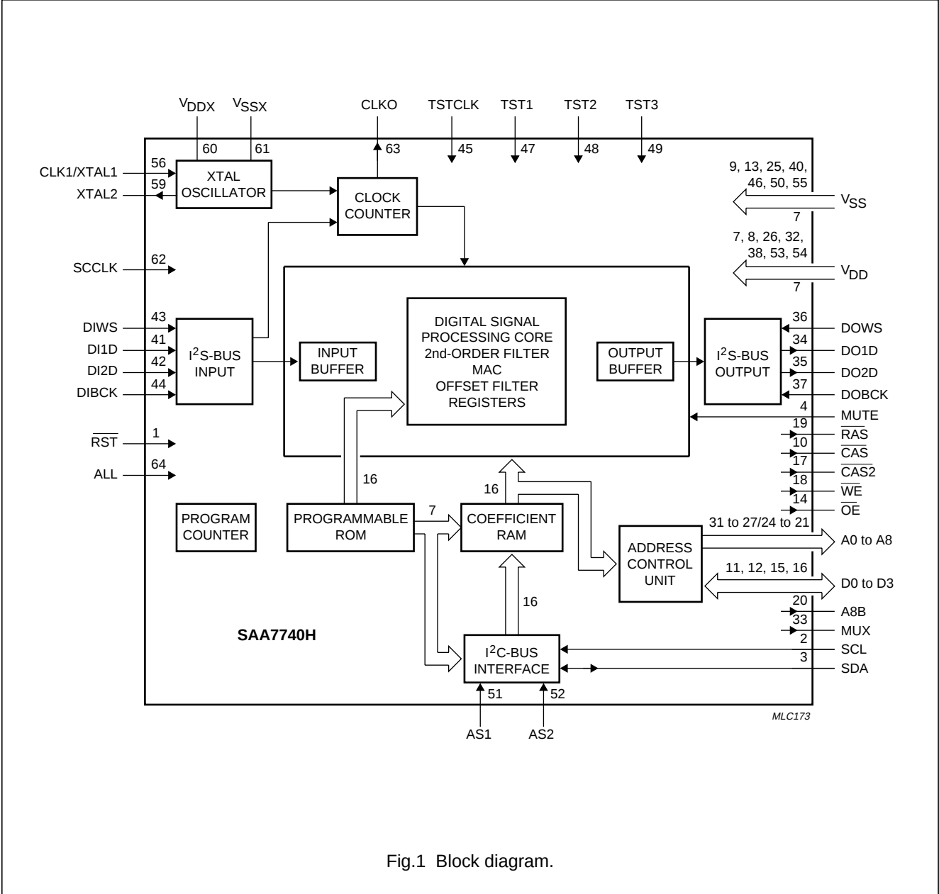
BLOCK DIAGRAM
