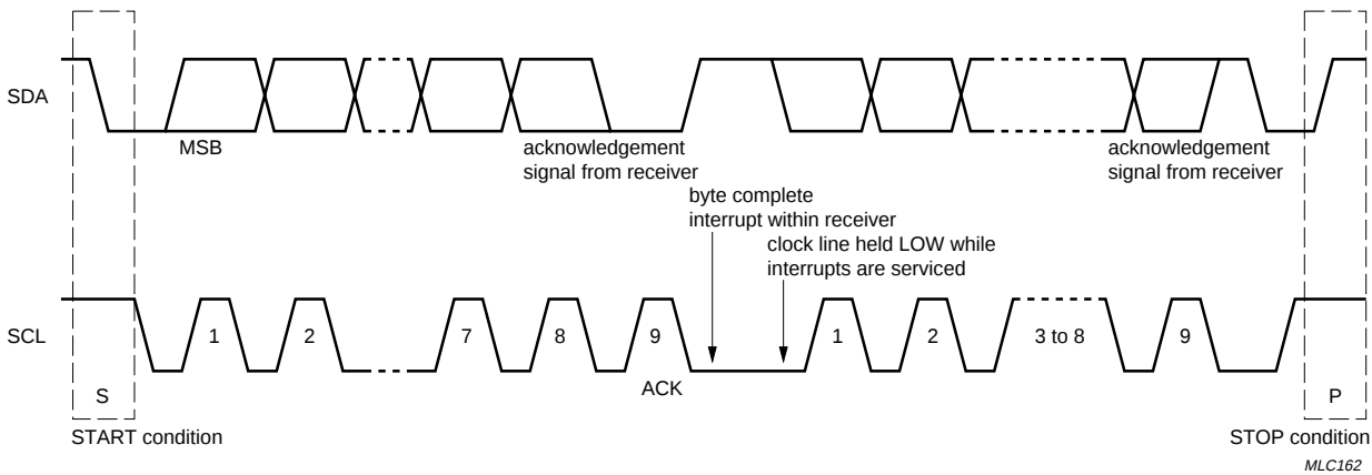
Fig.14 Data transfer on the I 2 C-bus.
