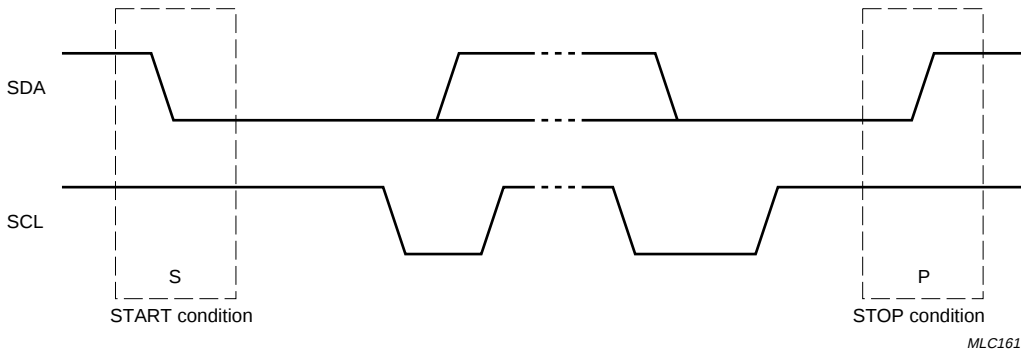
Fig.13 START and STOP conditions.
