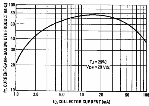
FIGURE 4 – CURRENT-GAIN-BANDWIDTH PRODUCT
