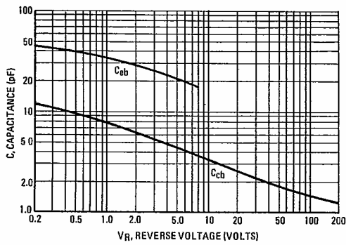
FIGURE 3 – CAPACITANCES
