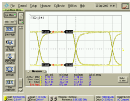
Bit rate: 2.5 Gb/s Vin = +/-200 mVpp, Vout = +/-672 mVpp
