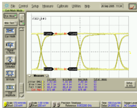
Bit rate: 2.5 Gb/s Vin = +/-50 mVpp, Vout = +/-672 mVpp
