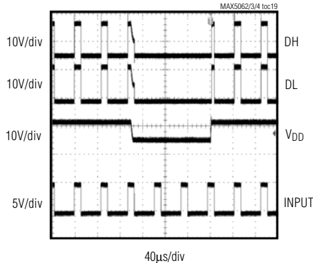
DH/DL RESPONSE TO V_{DD} GLITCH
