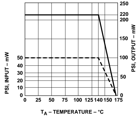
Figure 16. Dependence of Safety-Limiting Data on Ambient Temperature.
