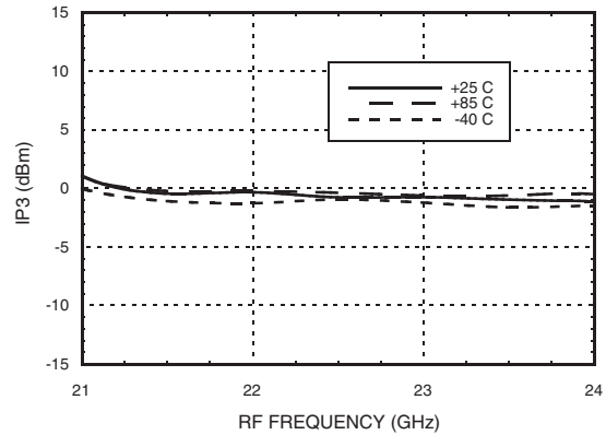
Input IP3, ULNB vs. Temperature
