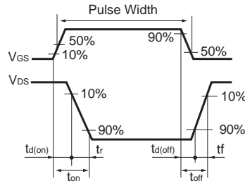
Fig.1-2 Switching Waveforms
