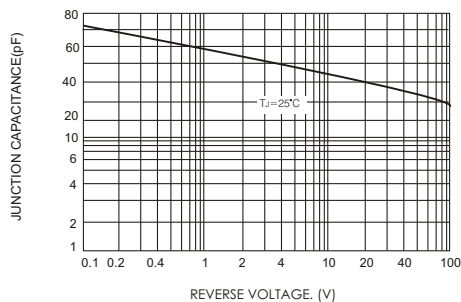
FIG.4-TYPICAL JUNCTION CAPACITANCE
