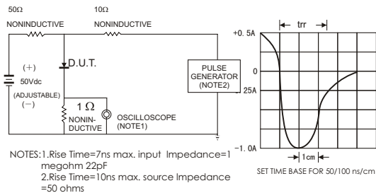
FIG.6-TEST CIRCUIT DIAGRAM AND REVERSE RECOVERY TIME CHARACTERISTIC
