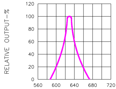
Fig.2 SPECTRAL RESPONSE
