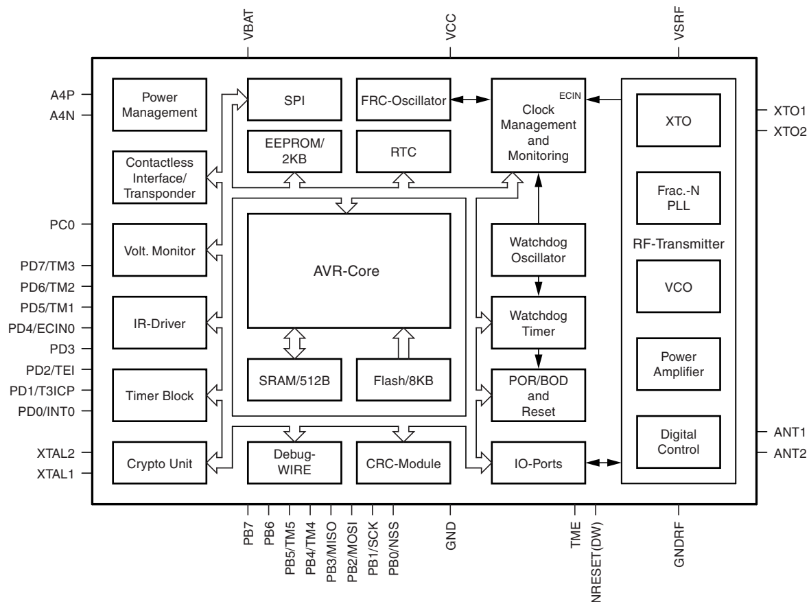
Figure 1-2. ATA5795 Block Diagram
