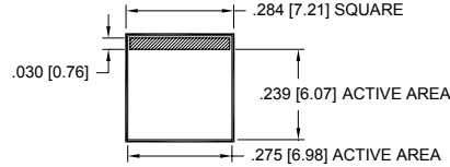
CHIP DIMENSIONS INCH [mm]
