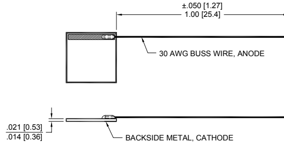
CHIP DIMENSIONS INCH [mm]
