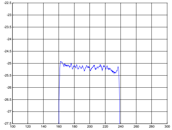
Phase Linearity(f0±37MHz)
