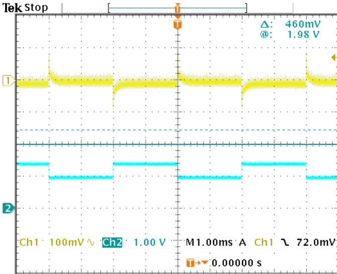
Fig 13. Dynamic response of load step at V_{in}=48v , Ch1: output voltage change(100mv/div), Ch2: output current step of 50%-75%-50% (1A/div). Current slew rate:0.1A/ \mu s, C_o=10\mu F tantalum capacitor + 1 \mu F Ceramic capacitor, time scale: 1ms/div
