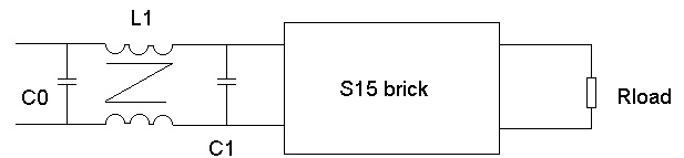
Fig 6A. The external filter circuit
